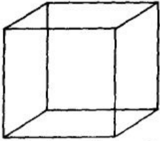
Necker Cube
